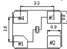
Recommended Solder Pattern
